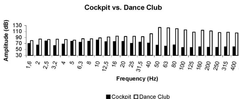
Figure 2. Frequency distributions, within the 1.6 – 500 Hz range, of the Airbus-340 cockpit in cruise flight and of a popular Lisbon Dance Club.
